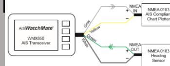
Optional chart plotter/radar and heading sensor
