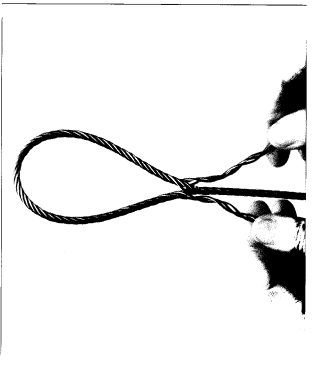
Lead strand and, if required, insert thimble. Pull each part back to and lay up together spalling round the standing part.
