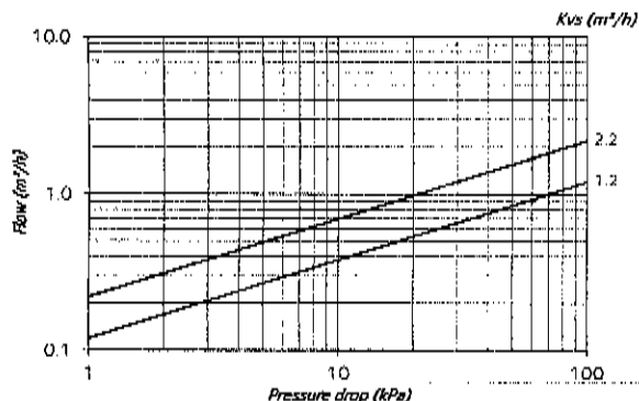
CAPACITY DIAGRAM
