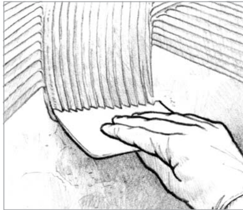
Figure 7 Apply the fairing compound with the notched spreader. Control the height of the ridges by the angle you hold the spreader.
