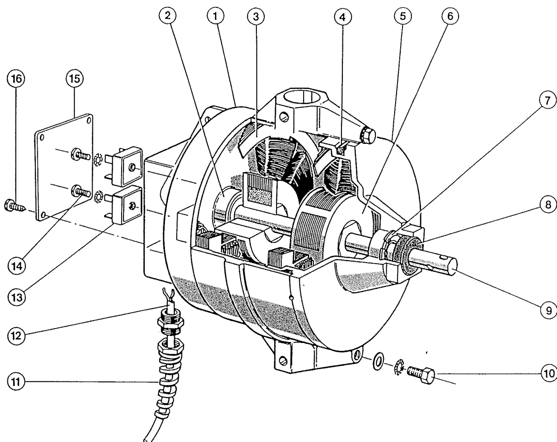
Figure 17. Sectioned Drawing.
