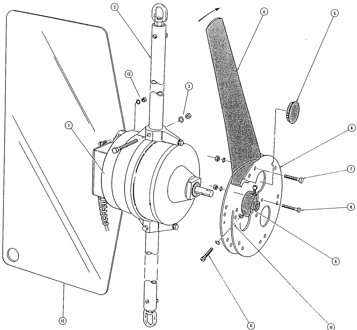
Figure 7. Aquair Wind kit Hoist in Rigging.
