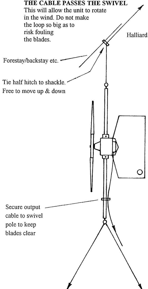
Figure 8. Aquair Hoist In Rigging mounting
