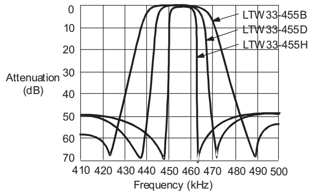
Frequency v. Attenuation Characteristics
