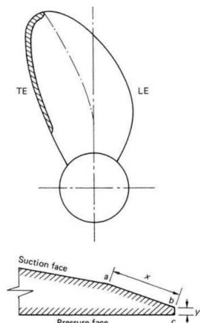
Figure 21.9 Anti-singing edge design
