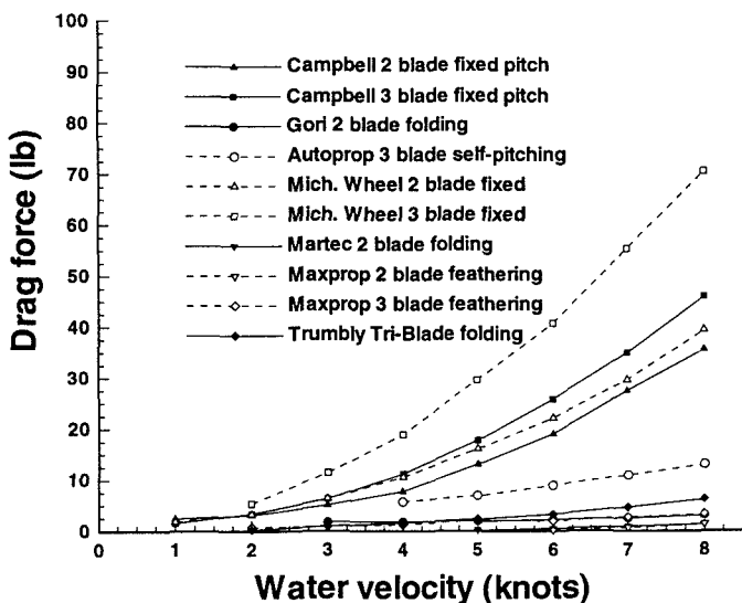
Fig. 14 Comparison of drag forces
