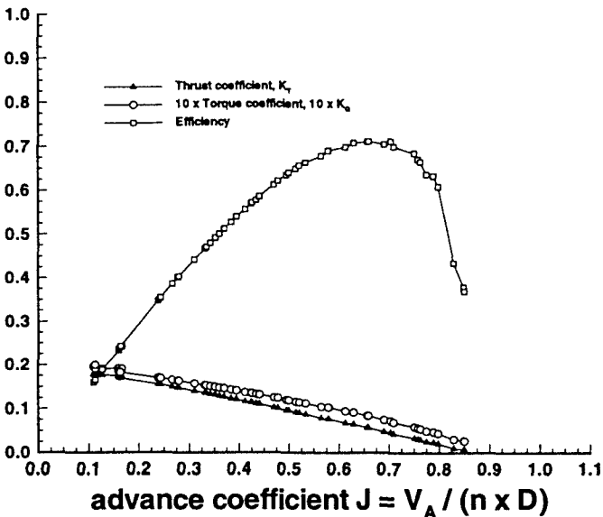
Fig. 2 Michigan Wheel 2-bladed 13 \times 10 fixed pitch
