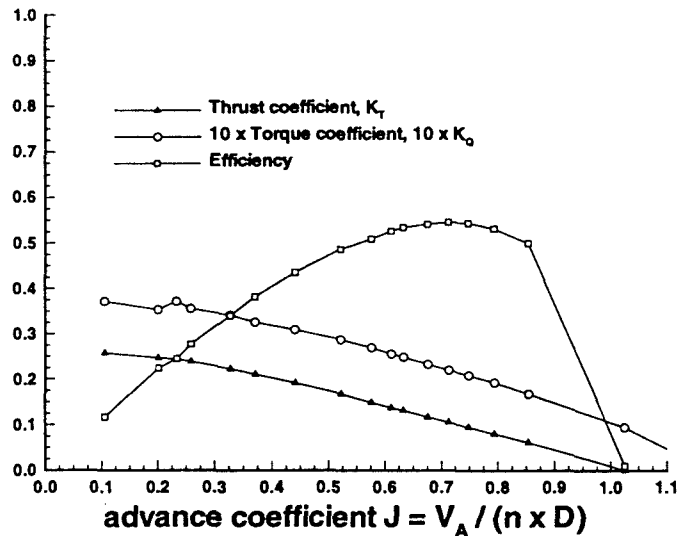
Fig. 4 Campbell 2-bladed 13 \times 10 fixed pitch
