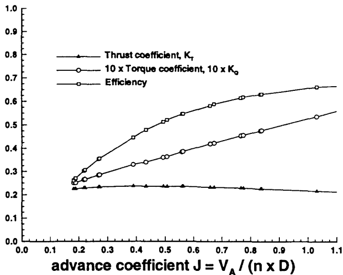
Fig. 10 Autoprop 3-bladed self-pitching, 13 in. diameter
