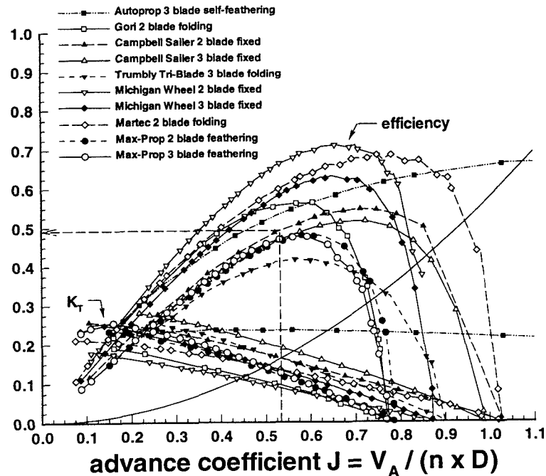
Fig. 12 Determination of propeller efficiencies
