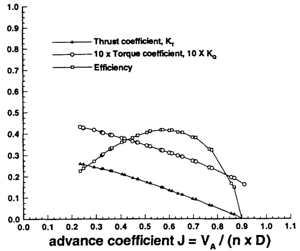
Fig. 11 Trumbly Tri-Blade 13 x 10 folding
