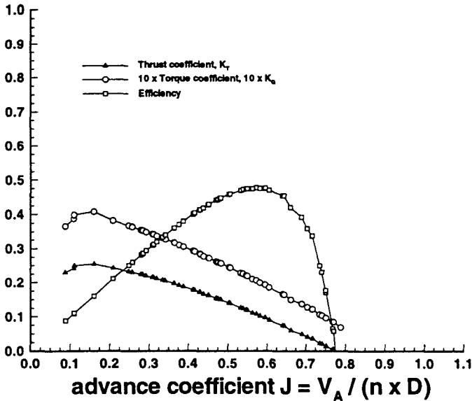
Fig. 9 Max-Prop 3-bladed 13 x 10 feathering
