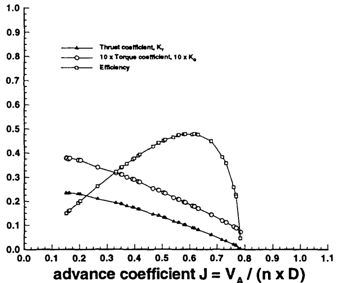
Fig. 8 Max-Prop 2-bladed 13 \times 10 feathering
