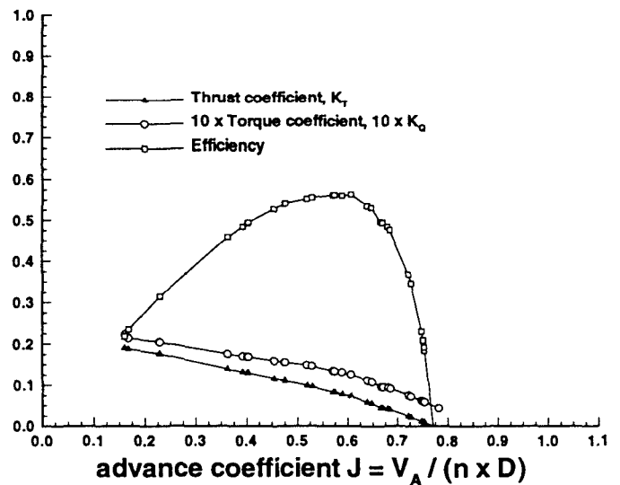
Fig. 7 Gori 2-bladed 13 \times 10 folding
