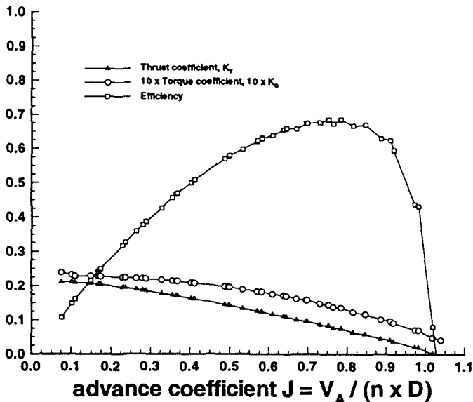
Fig. 6 Martec 2-bladed 13 \times 10 folding
