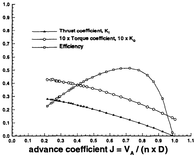
Fig. 5 Campbell 3-bladed 13 \times 10 fixed pitch
