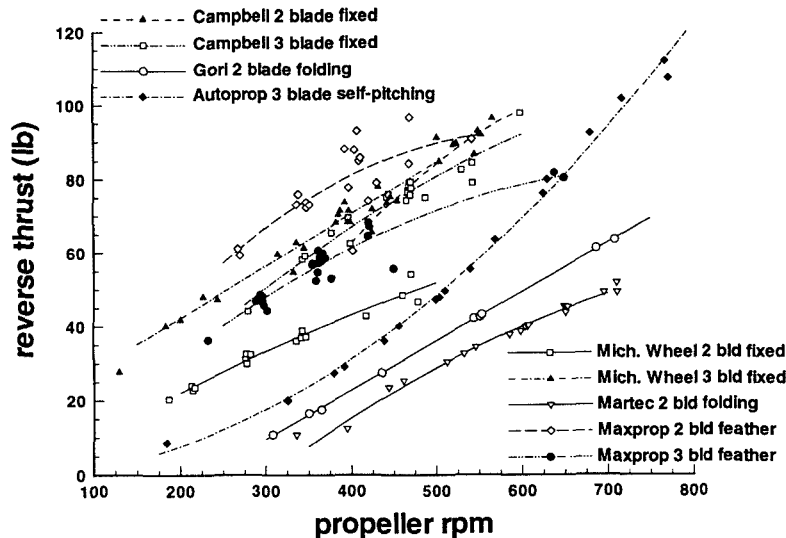
Fig. 13 Reverse thrust performance
