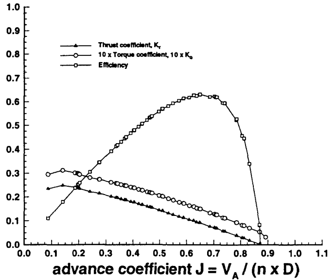
Fig. 3 Michigan Wheel 3-bladed 13 \times 10 fixed pitch
