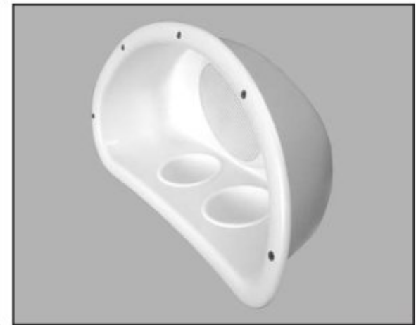
No. 54600300 128" (3251 mm) radius No. 54700300 52" (1321 mm) radius No. 56700300 38" (965 mm) radius 20 3/4"W x 10 1/2"H x 4 3/4" D (527 x 267 x 121 mm)
