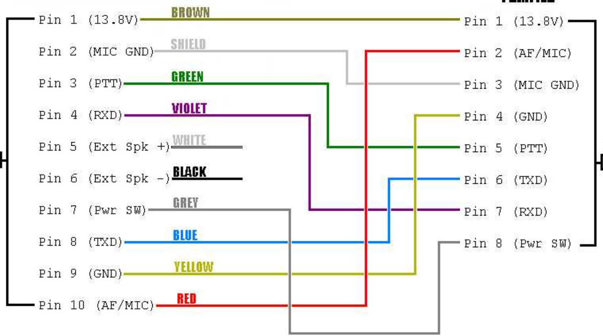
23 FOOT INTERCONNECT CABLE
