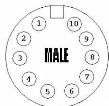
Interconnect Cable to MIC
