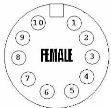
CMP25 Curly Mic Cable Pinout
