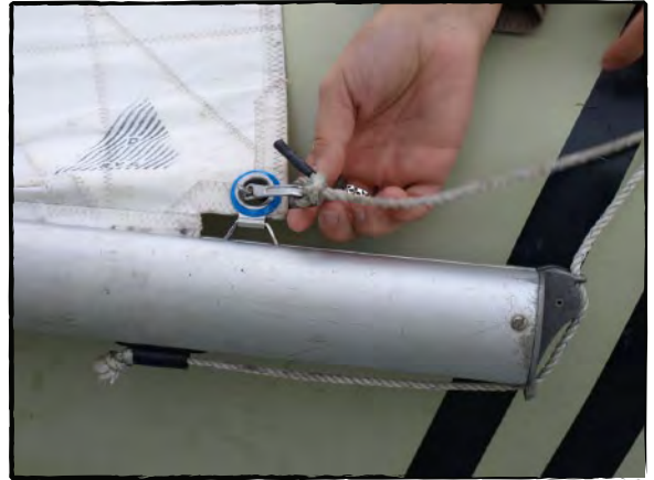
Photo 20, Attach to the sail, outhaul complete
