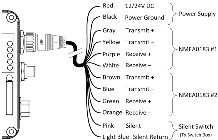
Figure 4 Wiring instructions
