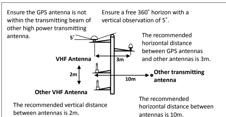
Figure 2 VHF/GPS antenna locations
